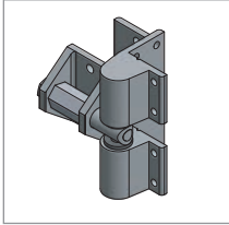
HD Adjustable Hinge for 2" Gate Side
