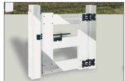
Post & Rail Vinyl Gate with Aluminum Reinforced Frame
